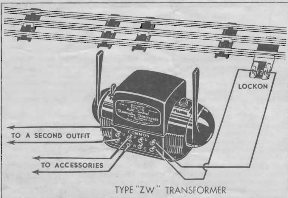
Figure 2—How to Connect the Transformer to Track.
